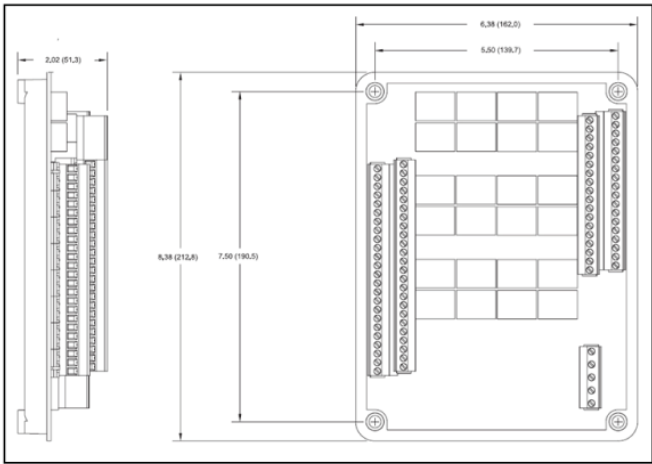
CEM-2020 Overall Dimensions
