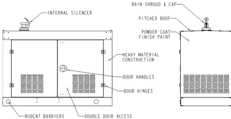
30 kW Enclosure Level 1
