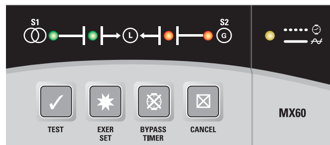
MX60 Microprocessor Control Panel
